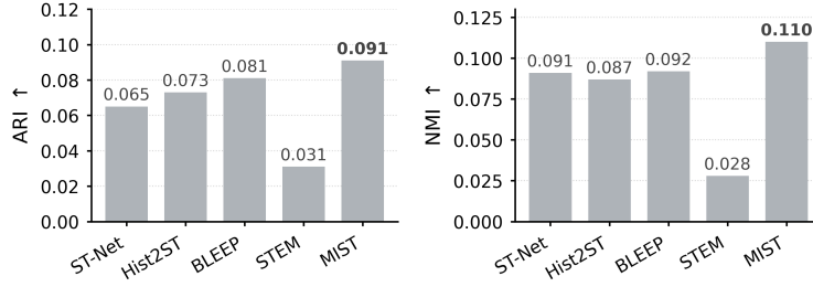
Figure 3: Spatial-domain recovery across all methods. Mean ARI (left) and NMI (right) (KMeans, k=6 ; predicted vs. measured domains); robustness to k is in Appendix I.
