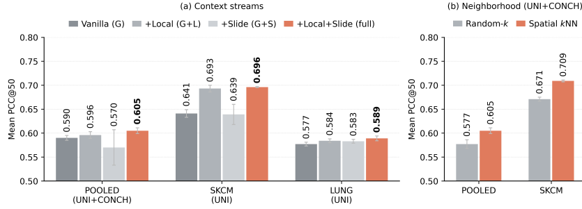
Figure 2: Context-stream ablation: self-attention is the vanilla Transformer backbone; local and slide are the added levers. (a) Context Streams. (b) Neighborhood.
