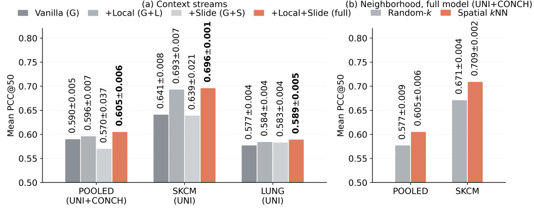
Figure 2: Context-stream ablation: self-attention is the vanilla Transformer backbone; local and slide are the added levers. (a) Backbone (Vanilla, G) plus the local and/or slide pathways, across POOLED (UNI+CONCH) and SKCM/LUNG intra-cohort (UNI). (b) Full model with spatial k NN vs. random- k neighbors (UNI+CONCH); spatially defined neighborhoods are significantly better. Bars are mean \pm std over three seeds.
