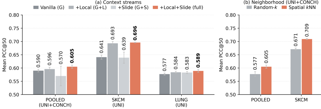
Figure 2: Context-stream ablation: self-attention is the vanilla Transformer backbone; local and slide are the added levers. (a) Context Streams. (b) Neighborhood.
