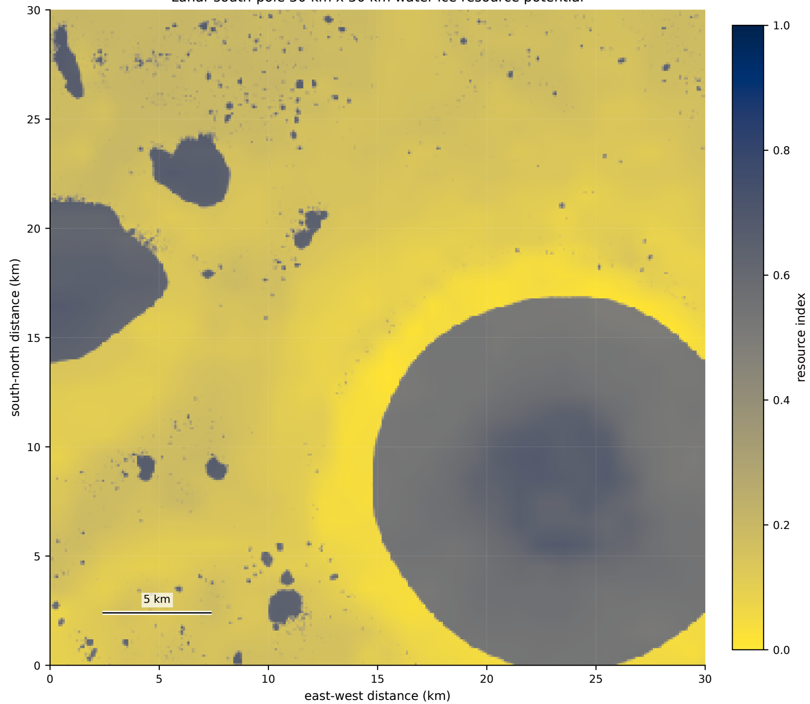
Lunar south-pole 30 km x 30 km water-ice resource potential
