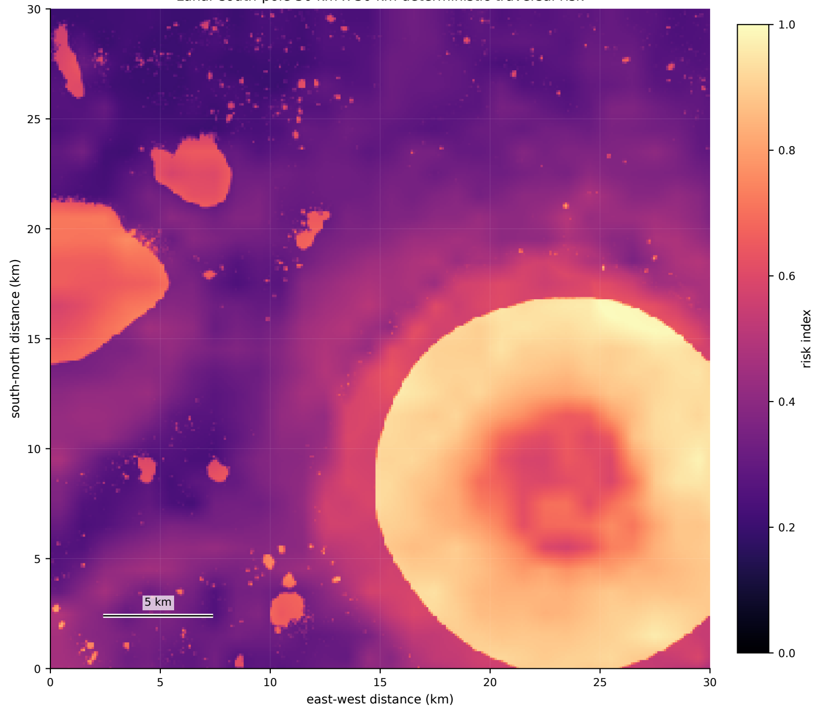
Lunar south-pole 30 km x 30 km deterministic traversal risk
