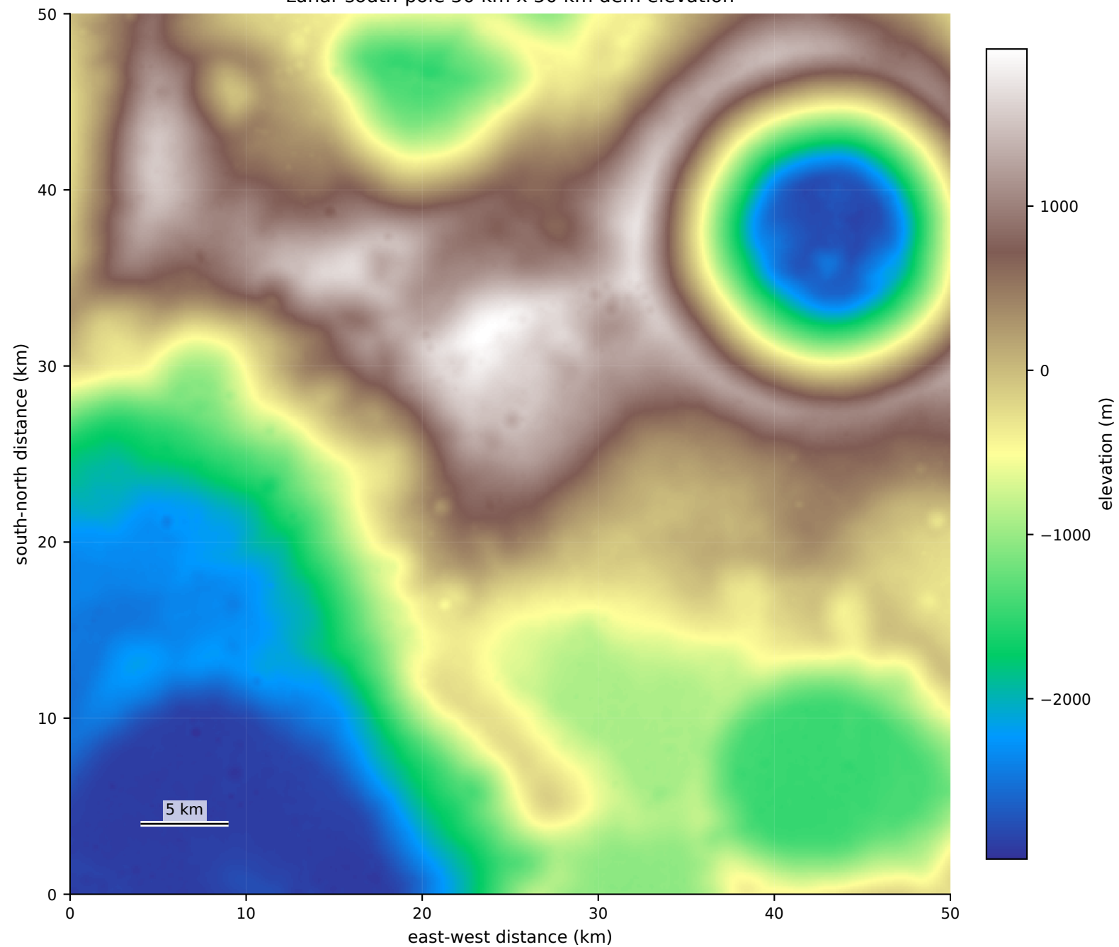
Lunar south-pole 50 km x 50 km dem elevation
