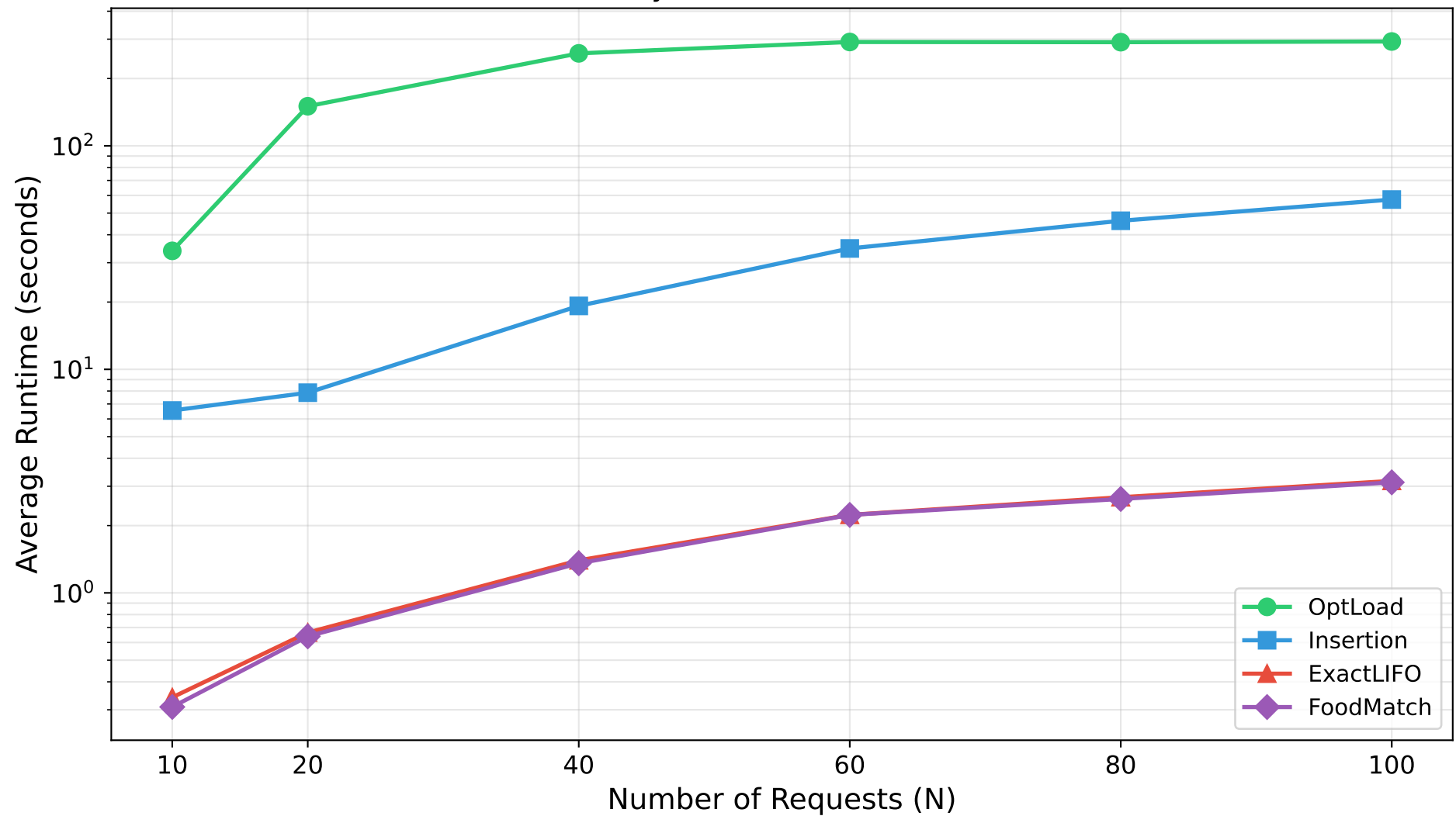
Scalability: Runtime vs Problem Size
