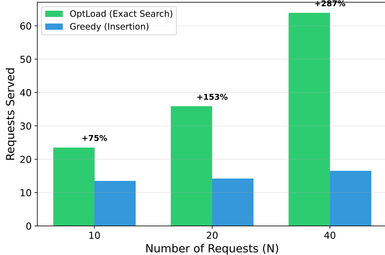
(a) Search Strategy Impact: Exact vs Greedy
