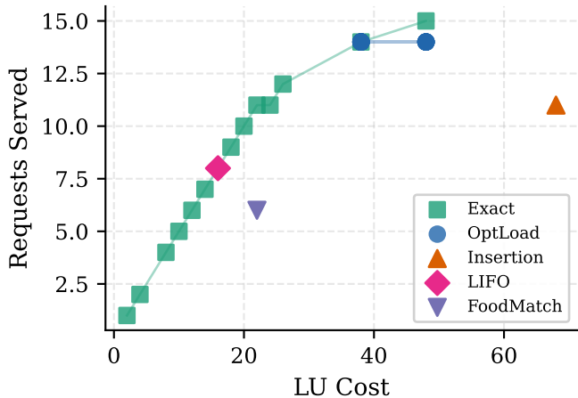
Pareto Front Example (N=5)
