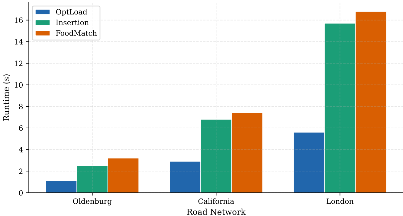
Figure 6: Runtime on Different Networks ( |R|=20 )
