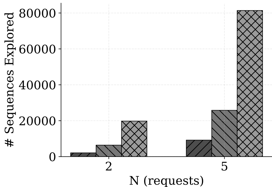
(b) Search-space size by ablation variant
