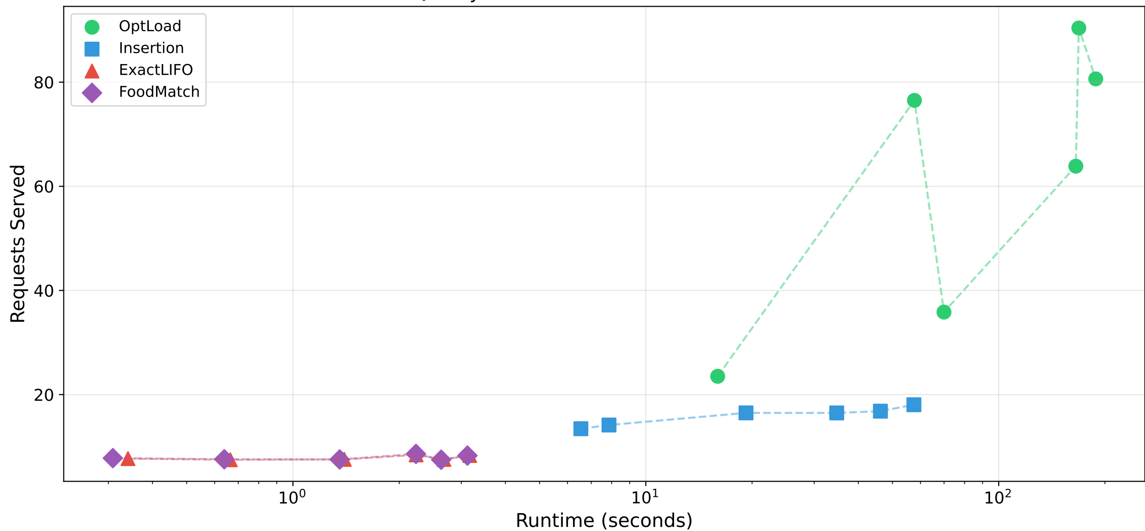
Quality-Time Trade-off: All Problem Sizes
