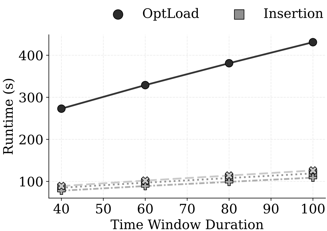
(a) Runtime vs Time Window
