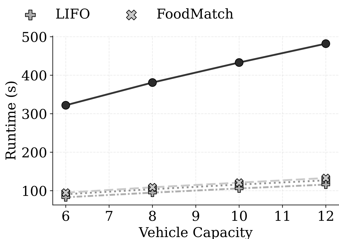
(b) Runtime vs Capacity
