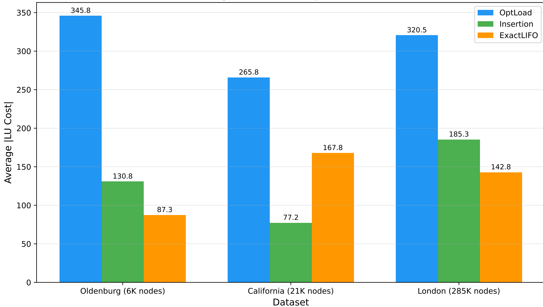
Network Scalability: LU Cost Comparison (Absolute Values)
