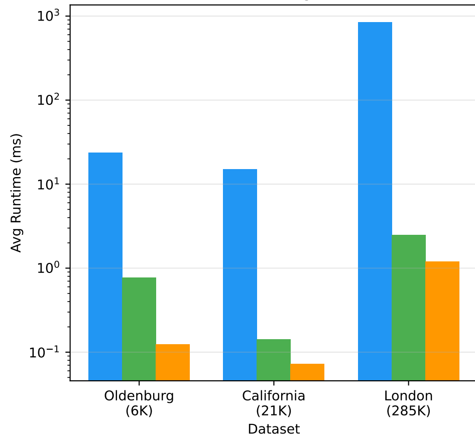
(c) Runtime (log scale)
