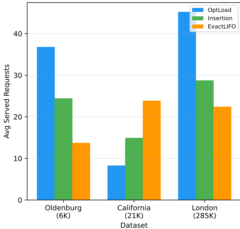
(a) Served Requests
