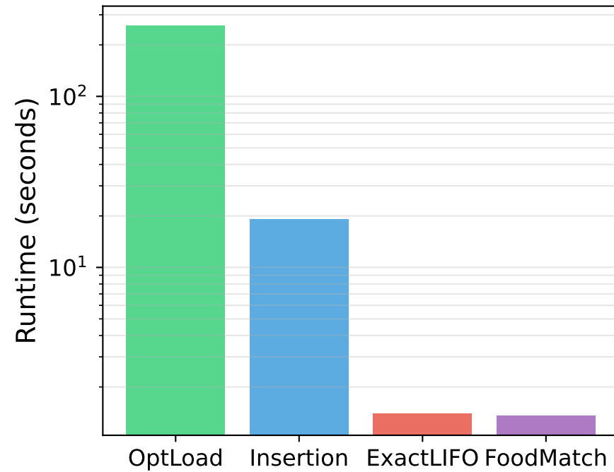
N=40: Runtime
