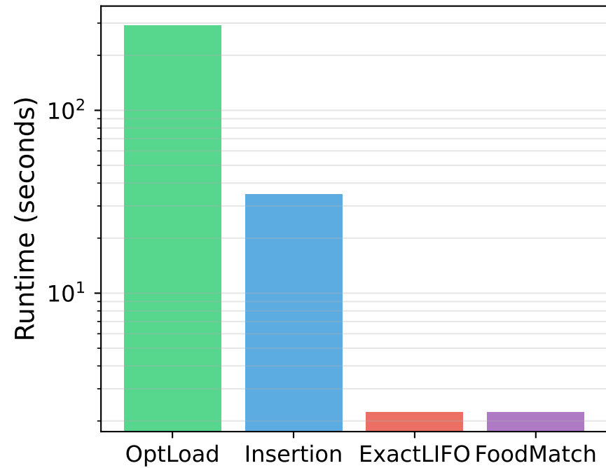
N=60: Runtime
