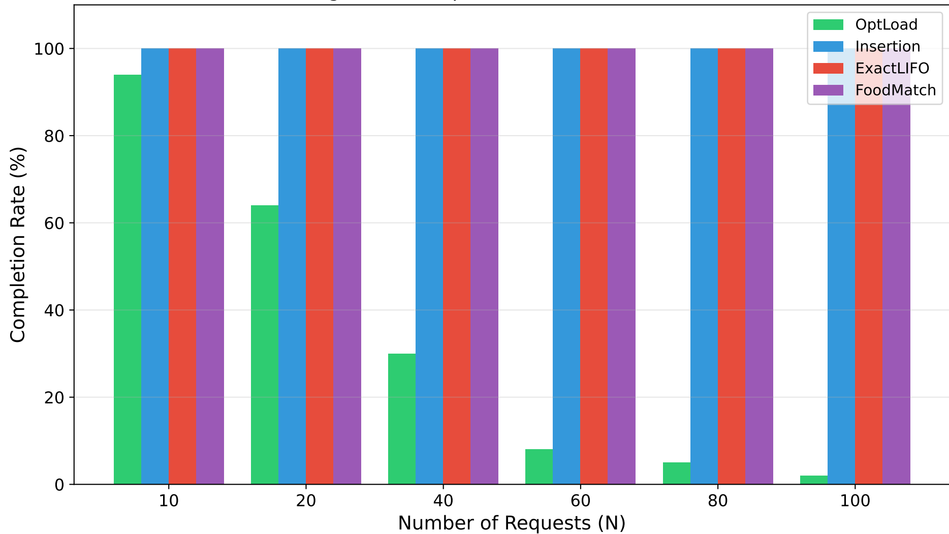
Algorithm Completion Rate (300s timeout)
