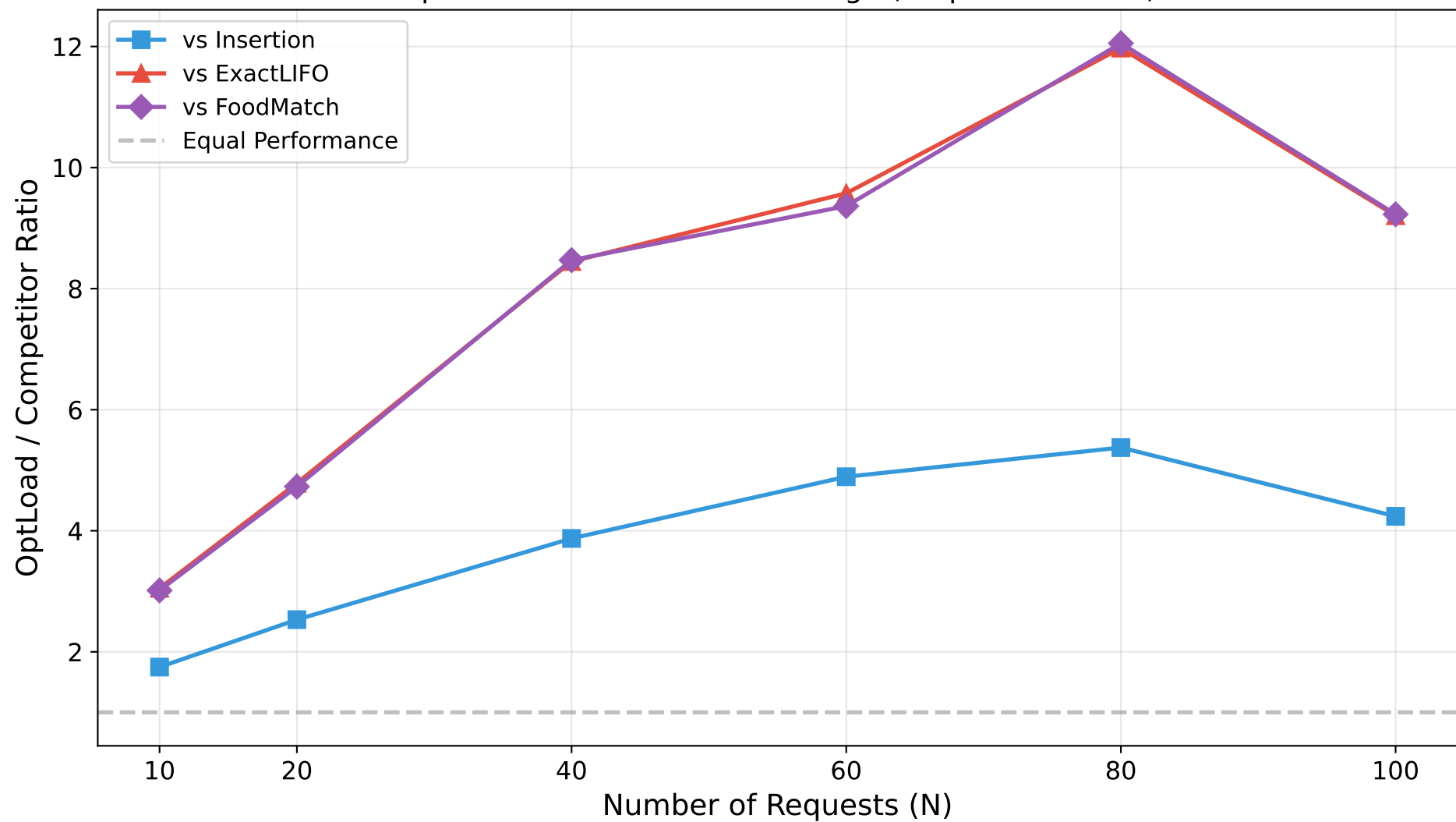
OptLoad Performance Advantage (Requests Served)
