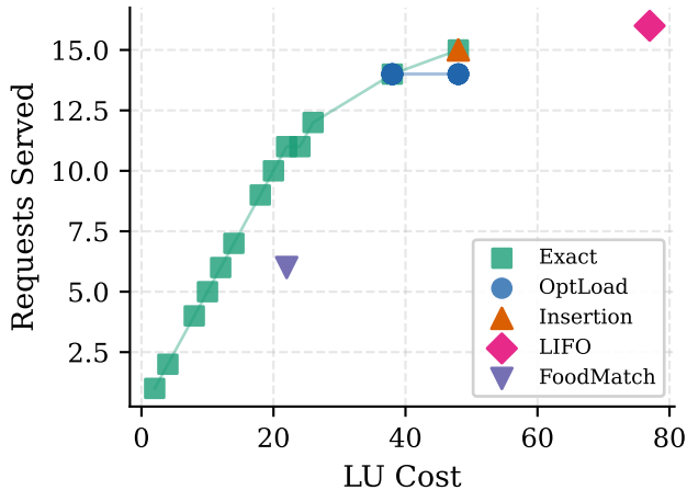
Pareto Front Example (N=5)
