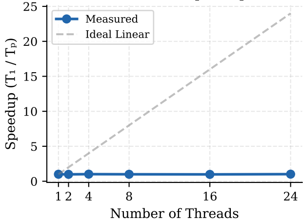
(b) Parallel Speedup
