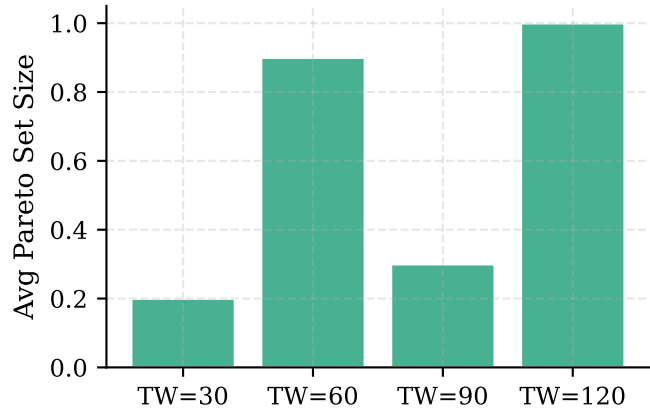
(b) Time Window \rightarrow Pareto Diversity
