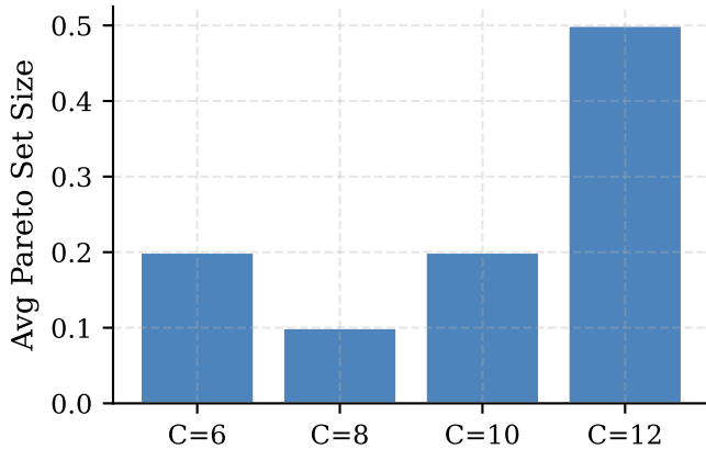
(a) Capacity \rightarrow Pareto Diversity
