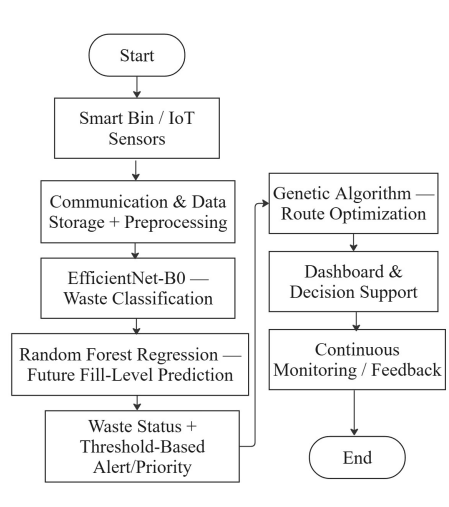
Figure 2: Flowchart of Ecosentinel
