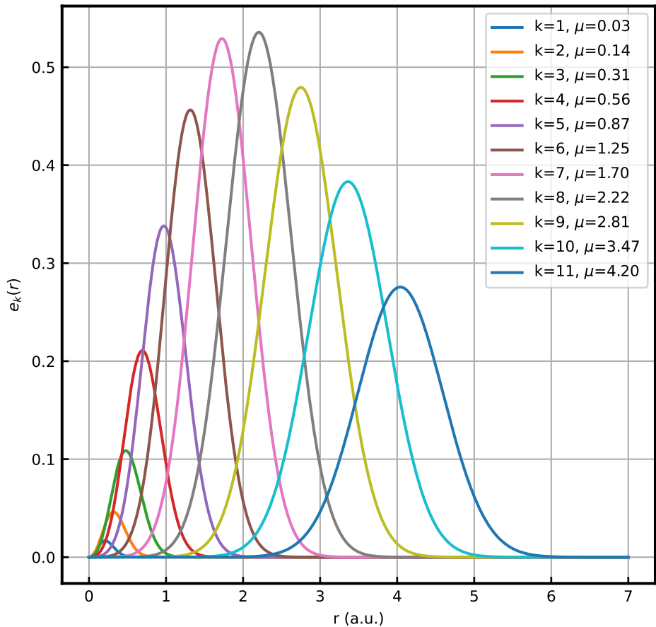
PauliNet RBF features vector ( K=11 , r_c=5.0 )
