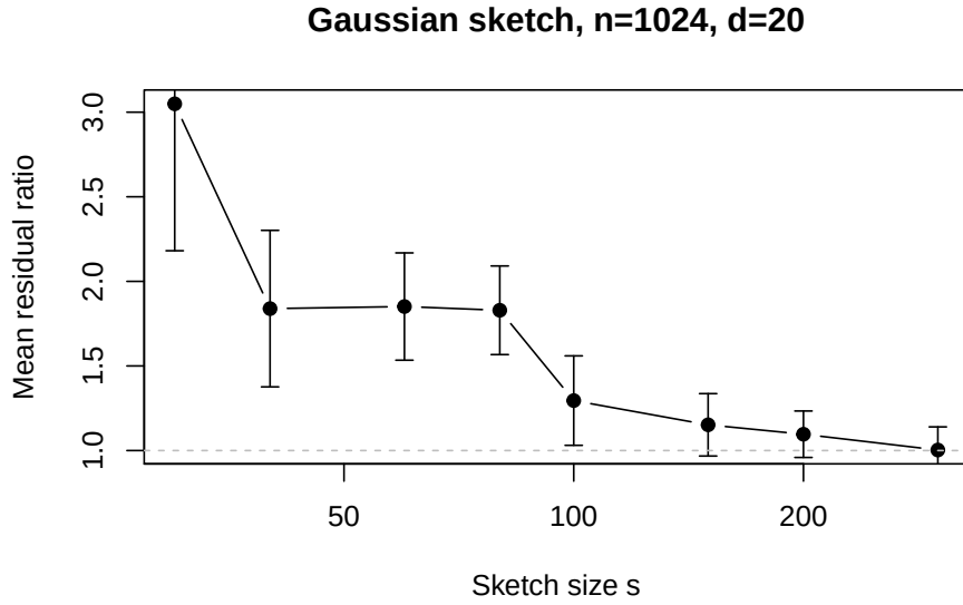
Figure 5.1: Mean residual ratio versus sketch size for Gaussian sketching of a noisy least-squares problem with n = 1024 , d = 20 . Error bars indicate one standard deviation across 20 independent trials.
