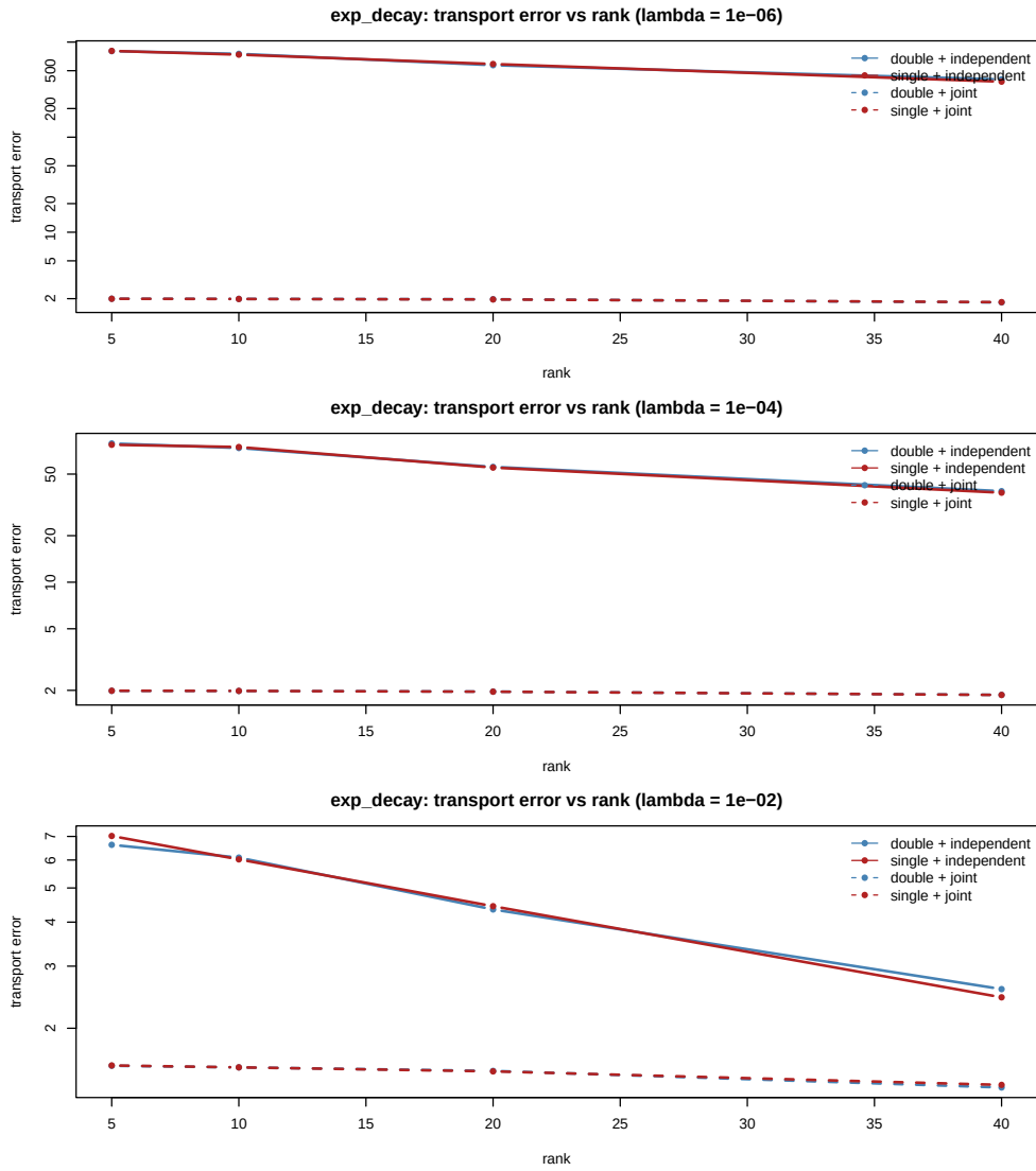
Figure 4 / Transport-map error versus rank. Regularization changes the picture decisively: with \lambda = 10^{-6} , the inverse-square-root amplification produces errors of order 10^2 to 10^3 , while with \lambda = 10^{-2} the transport error drops to order one and decreases further with rank.
