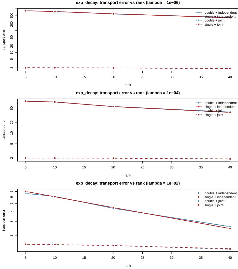
Figure 2 / Transport-map error versus rank. Regularization changes the picture decisively: with \lambda = 10^{-6} , the inverse-square-root amplification produces errors of order 10^2 to 10^3 , while with \lambda = 10^{-2} the transport error drops to order one and decreases further with rank.
