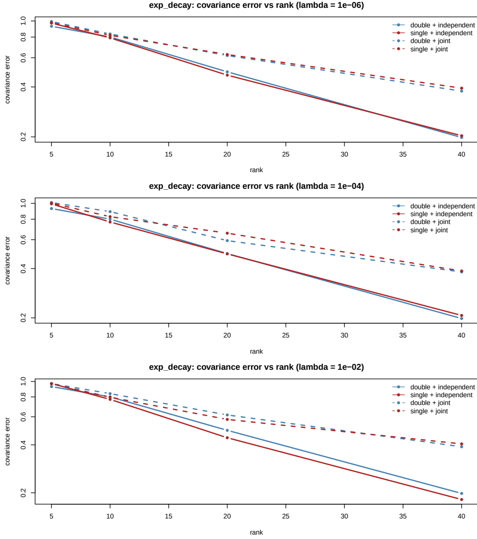
Figure 1 / Covariance approximation error versus rank on the focused synthetic latent-data validation. The error decreases consistently as the target rank grows, and simulated single precision remains close to double precision in this truncation-dominated regime.
