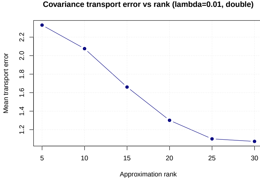
Figure 5.7: Mean absolute transport error versus target rank at fixed \lambda = 10^{-2} (exponential spectrum, p = 30 , double precision, Gaussian sketch).
