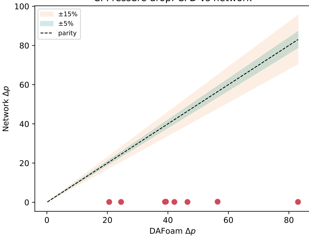
C. Pressure drop: CFD vs network
