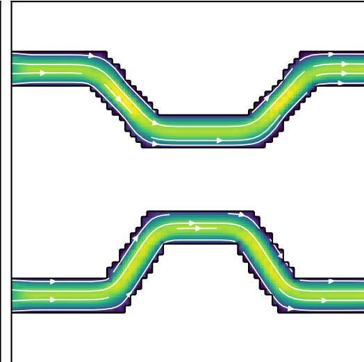
Relative |u| + streamlines
