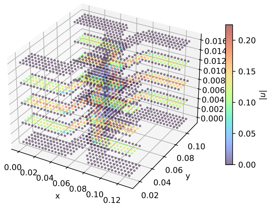
A. Extruded chamber fluid volume
