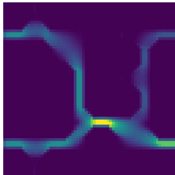
Finite-budget velocity: solver-distilled NN vs converged DAFoam
