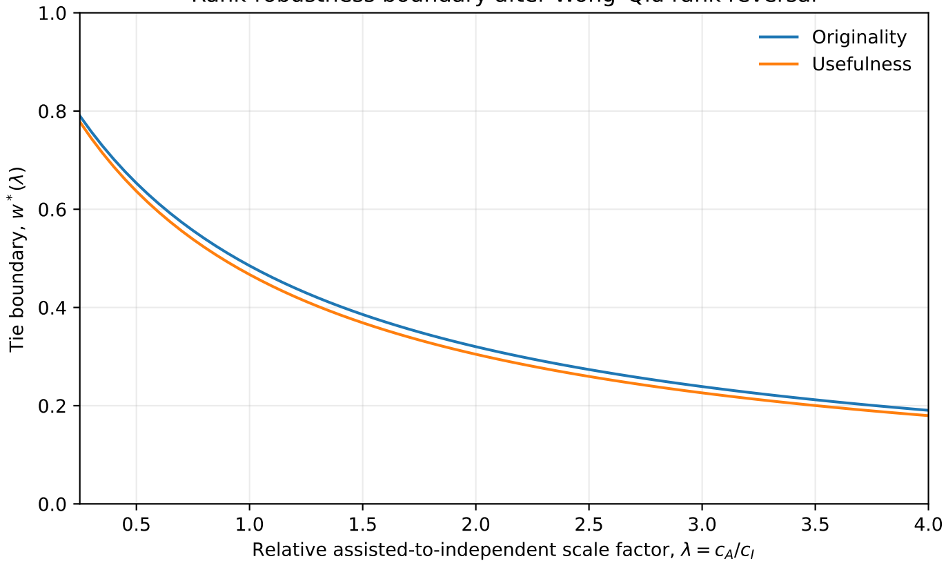
Rank-robustness boundary after Wong-Qiu rank reversal
