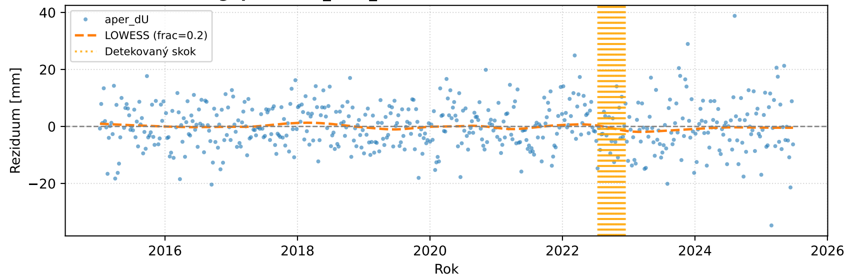
gop25wd04_stcd_licb - dU (k=2, min=3.0 mm/rok)
