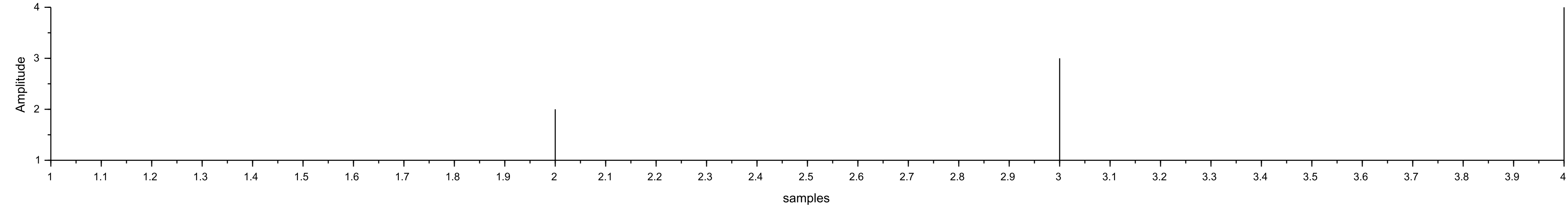
Linear Convolution of signals
