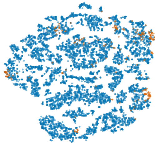
perplexity=50
