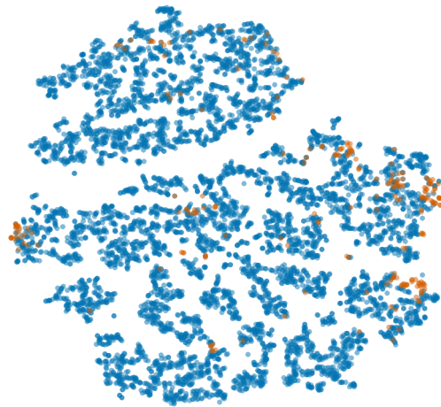
perplexity=30
