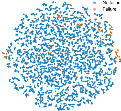
perplexity=5
