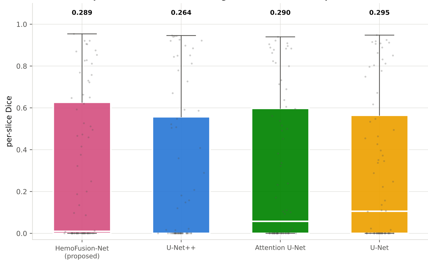
Distribution of per-slice Dice on hemorrhagic test slices (mean printed above each box)
