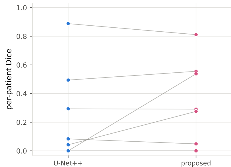
U-Net++ · proposed better on 3/15 patients
