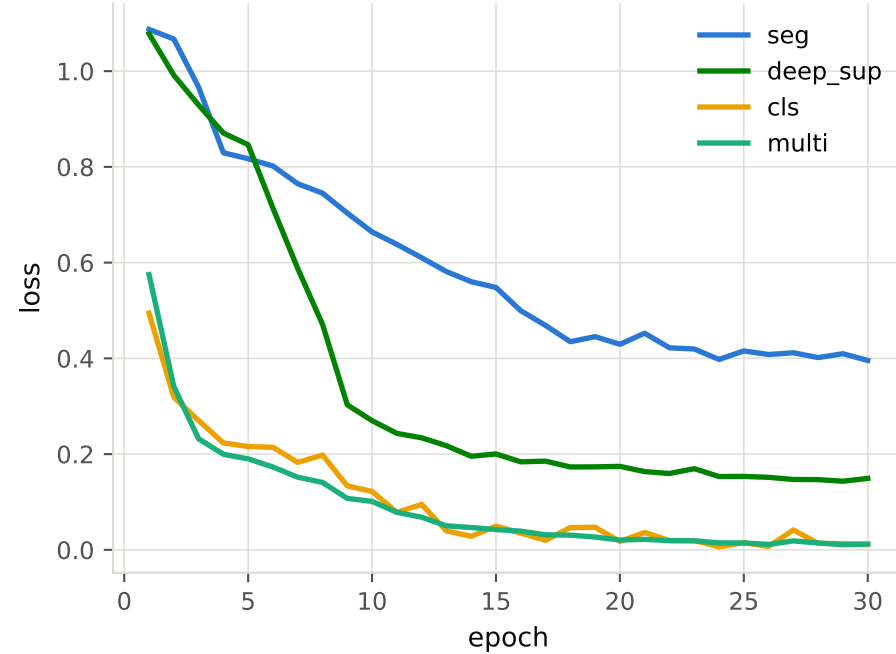
Loss components (train)
