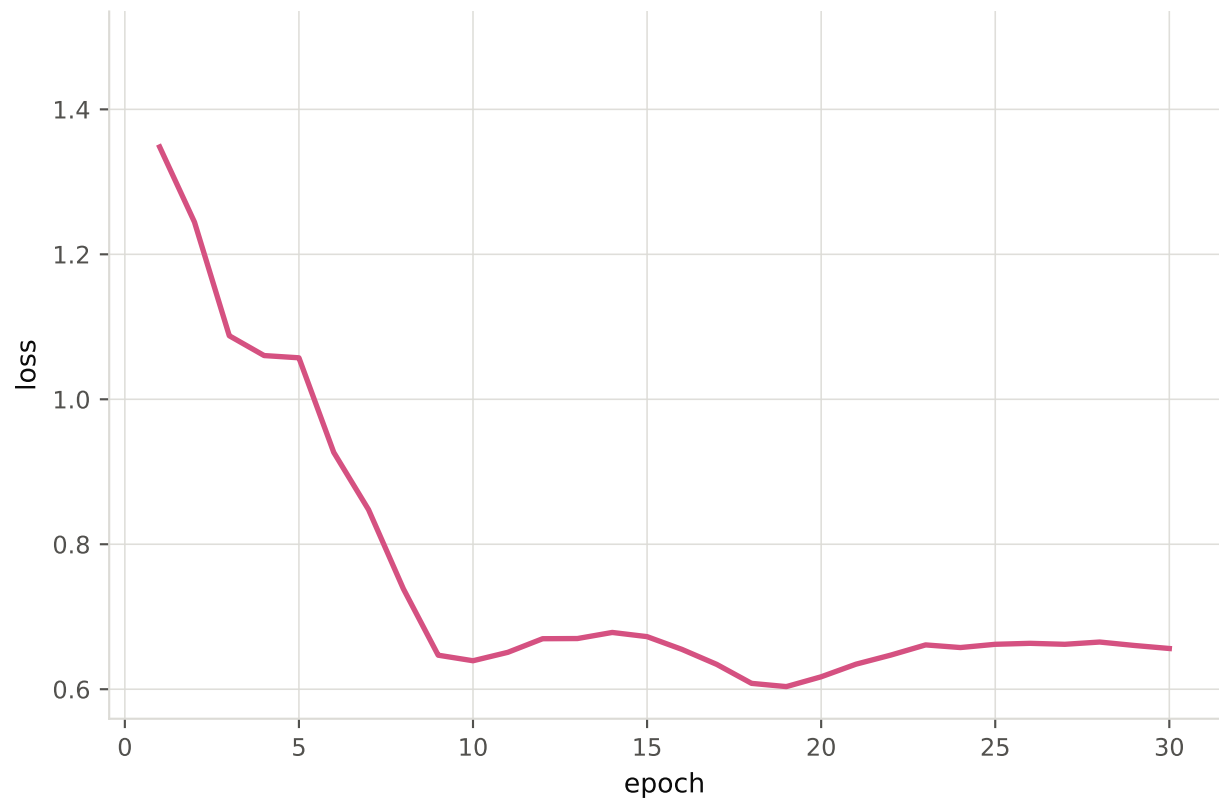
Validation loss
