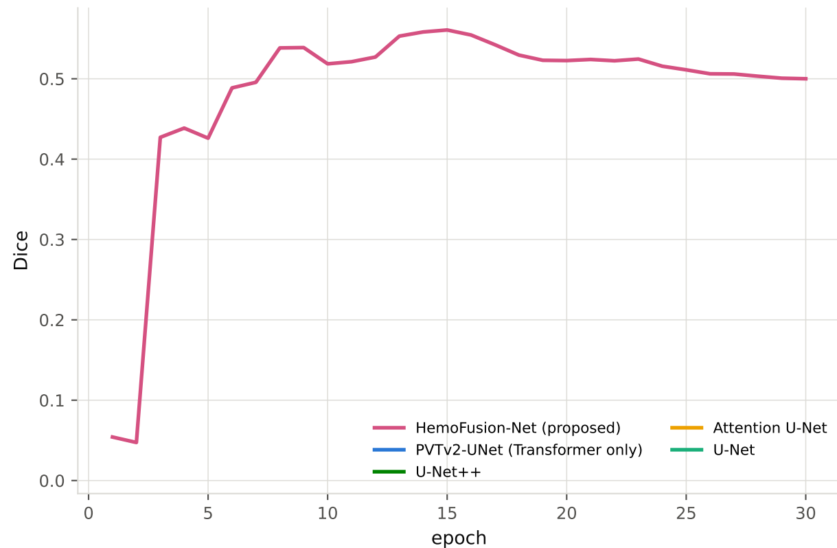
Validation Dice
