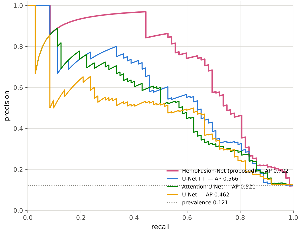
Precision-recall
