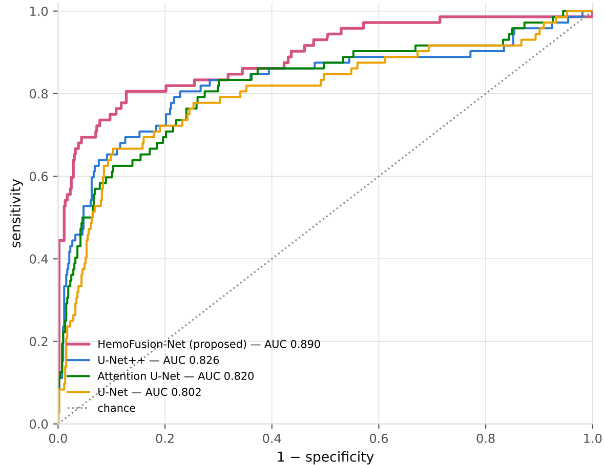
ROC — slice-level hemorrhage detection
