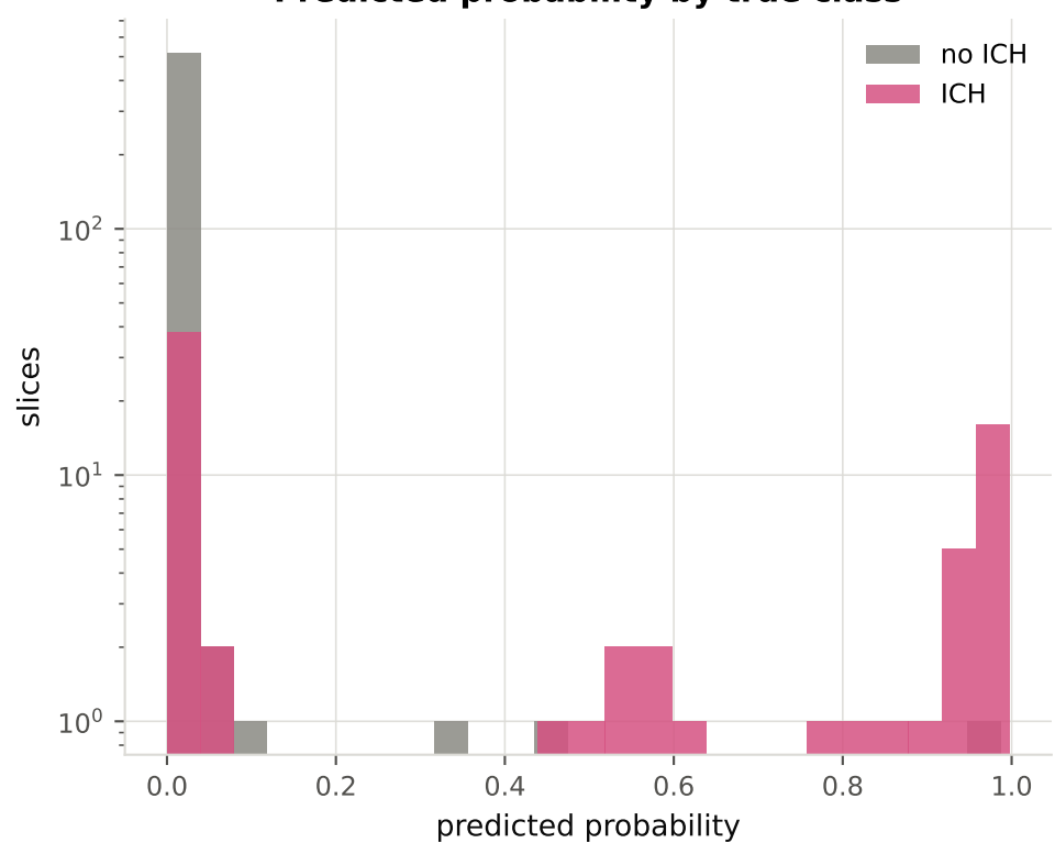
Predicted probability by true class
