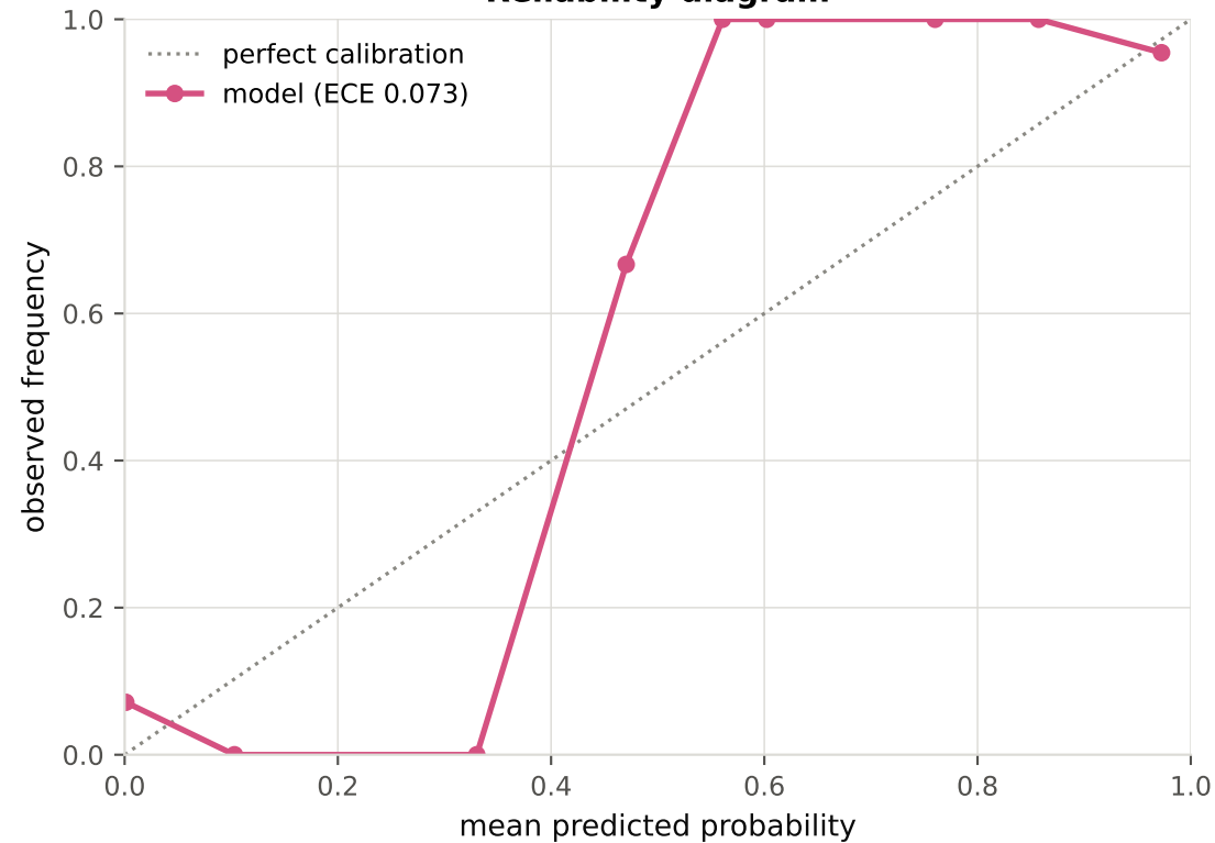
Reliability diagram
