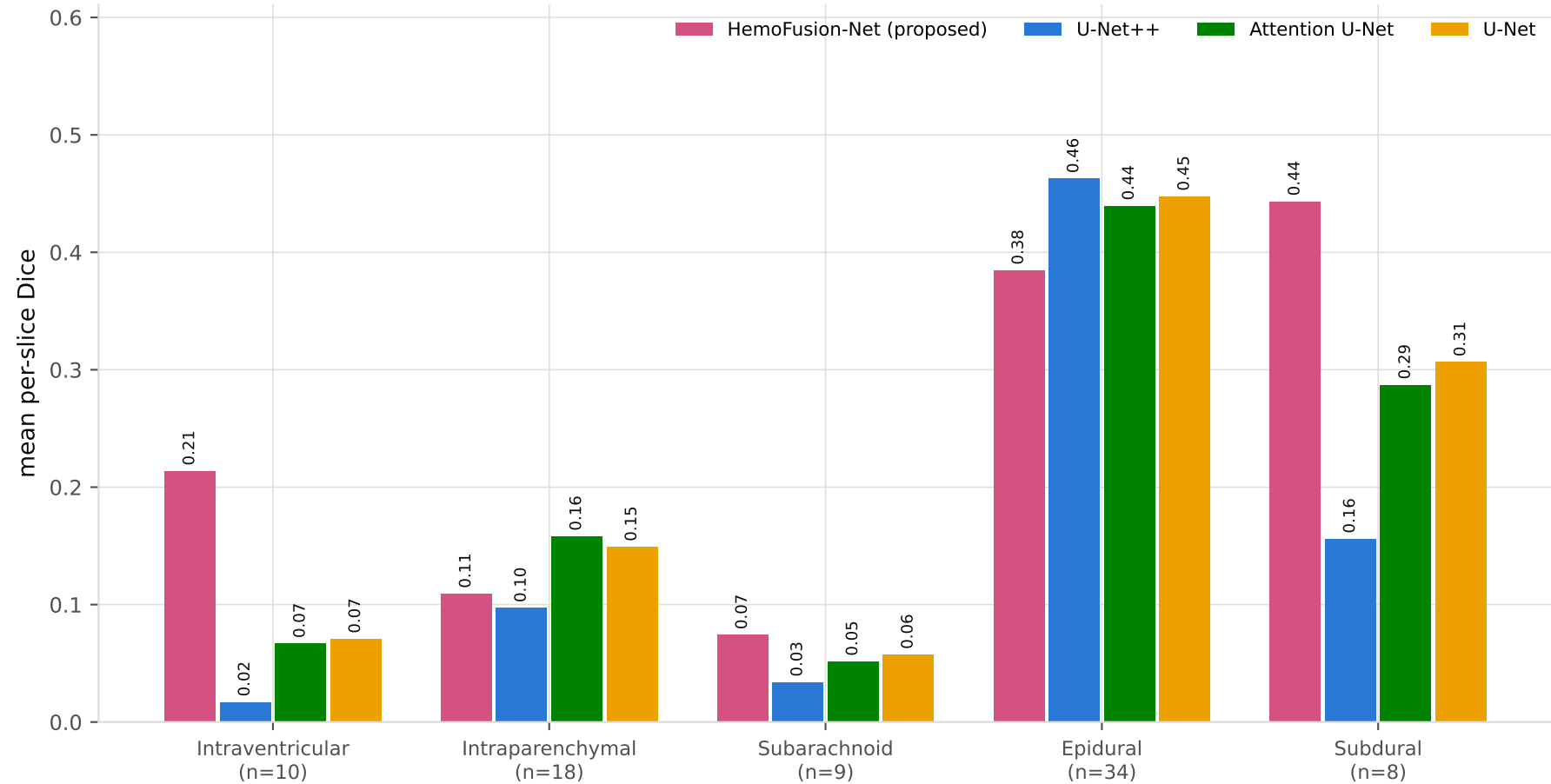
Class-wise segmentation performance (Dice)
