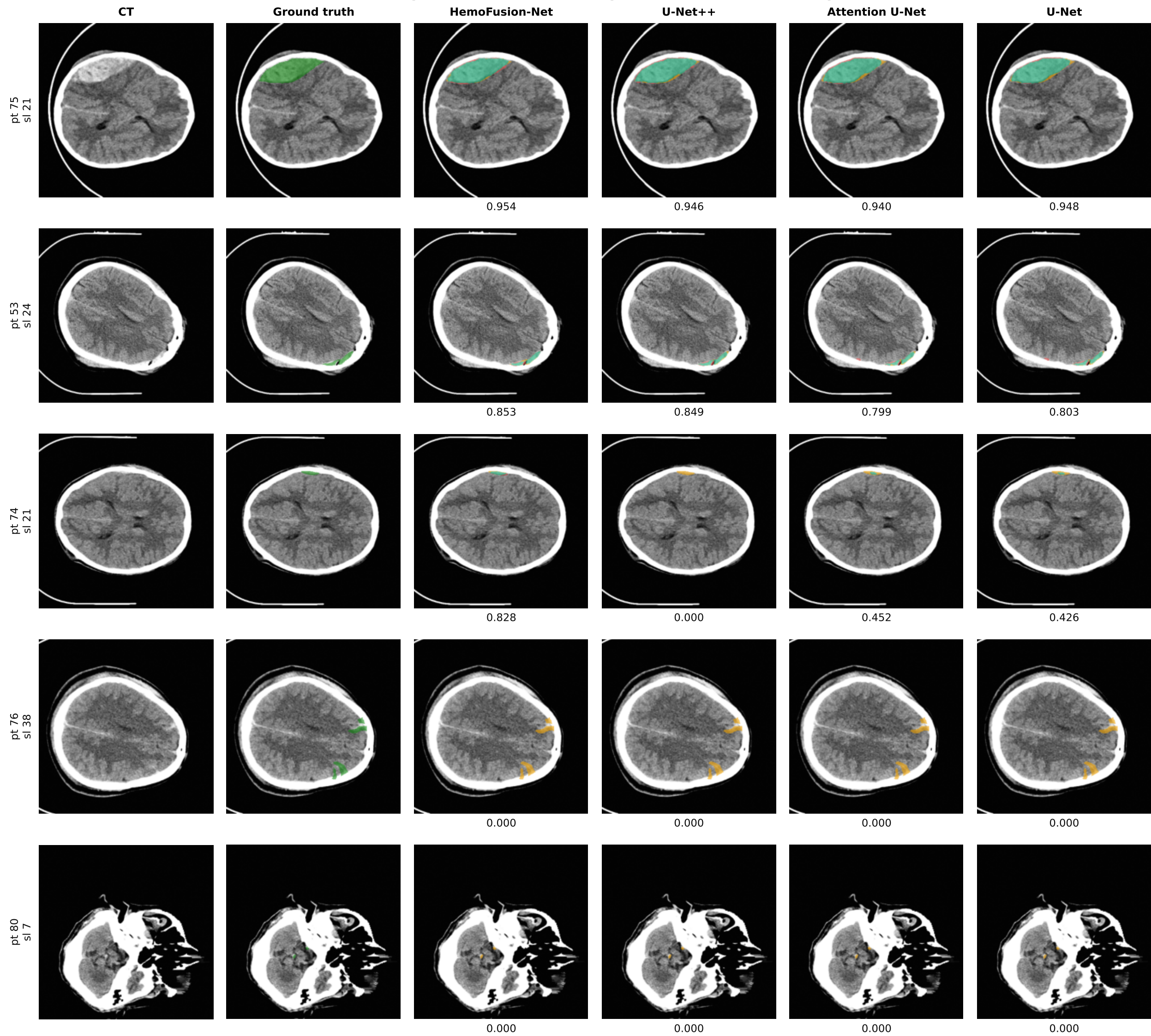
Qualitative comparison across models (per-slice Dice below each panel)
