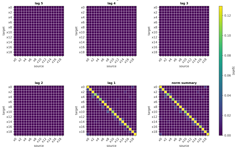
Xneural VAR causal gate: Lorenz-96 F=40
