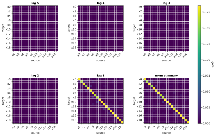
Xneural VAR causal gate: Lorenz-96 F=10
