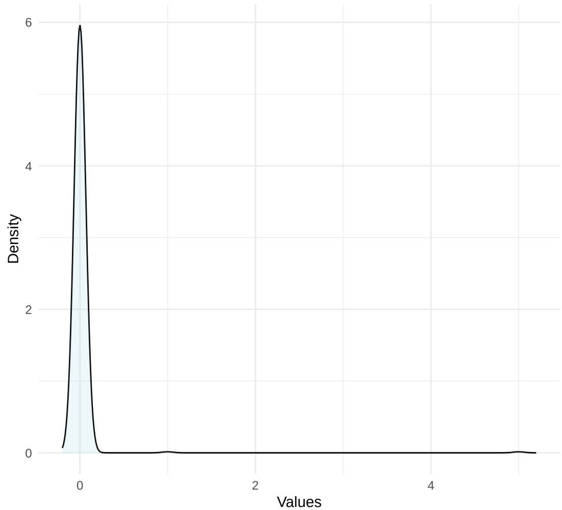
Density Plot for d.
