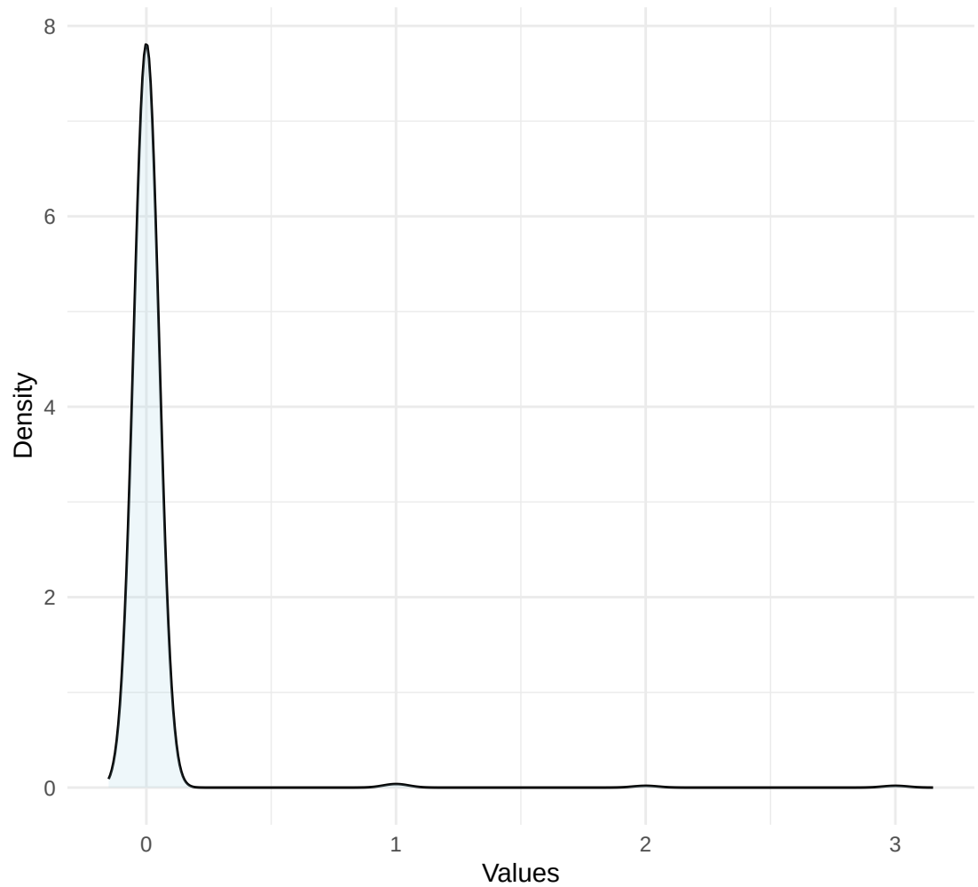
Density Plot for e.
