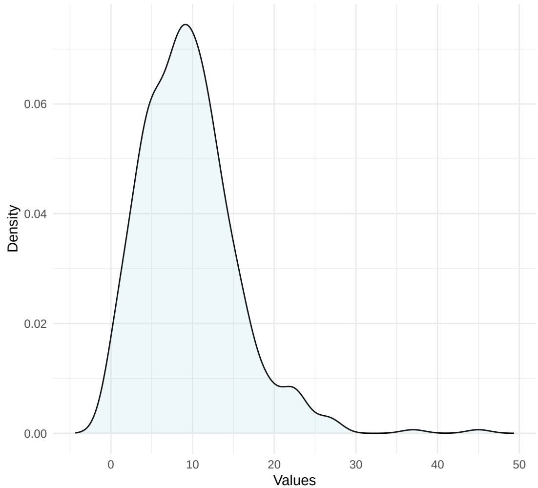
Density Plot for g
