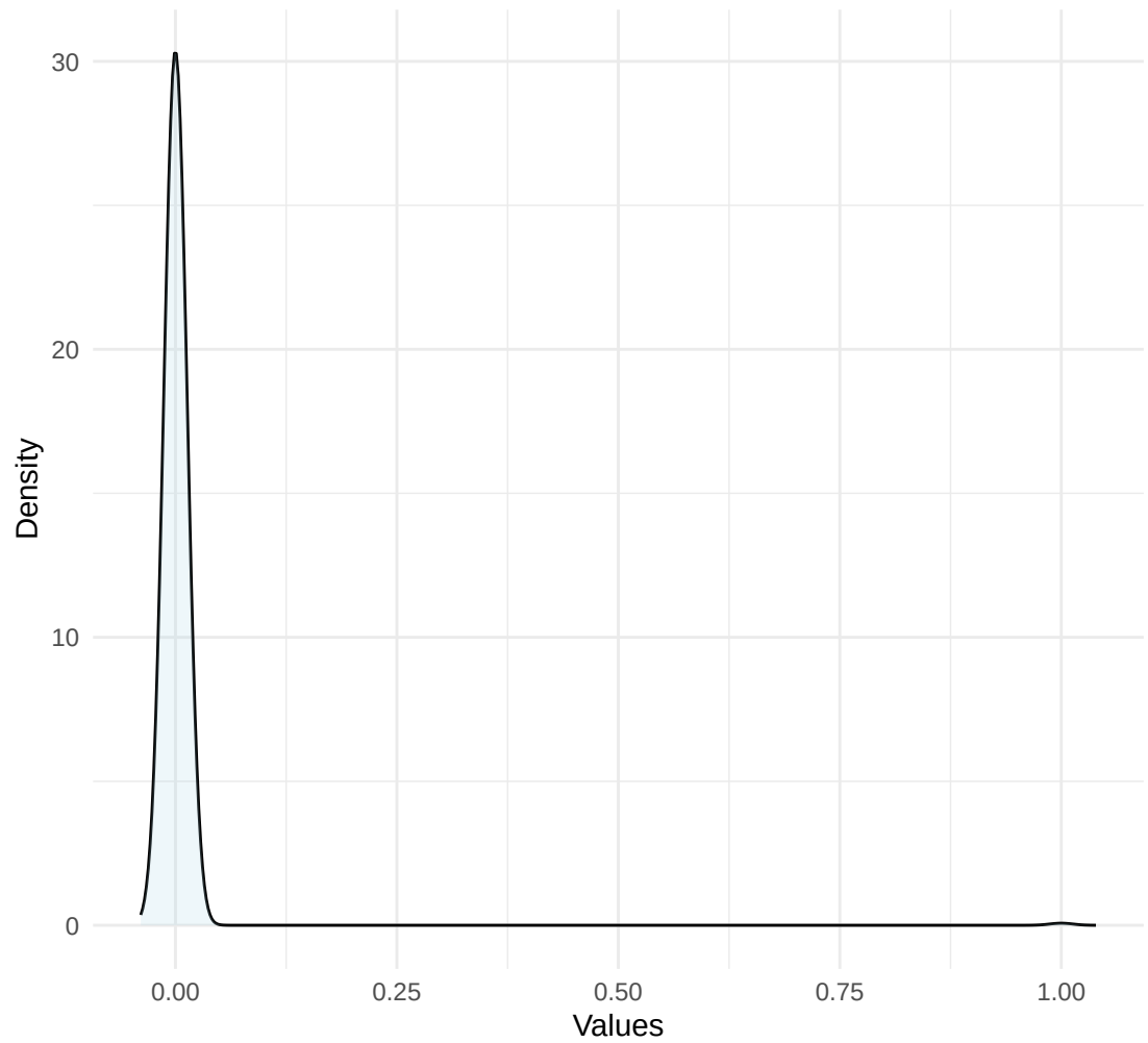
Density Plot for p.
