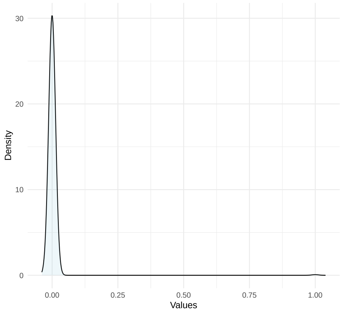
Density Plot for q .
